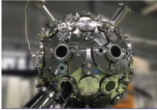
Laser Compressor Chamber
