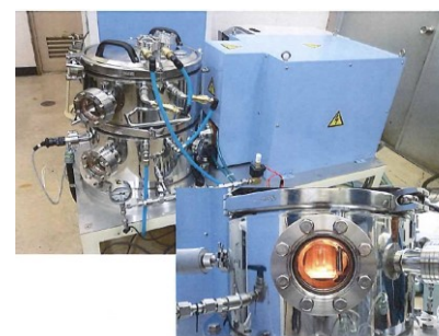
Welding process in manufacturing chambers
