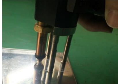
〈Step 2〉 Press CD weld gun at a position at which welding is to be performed...
